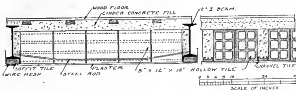
DETAILS OF FLOOR CONSTRUCTION
